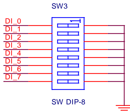
Figure 5. DI Switch of the WIZ220IO Base Board
