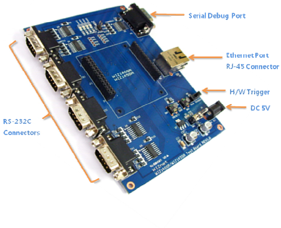
Figure 3. WIZ140SR/WIZ145SR Test Board Interface
